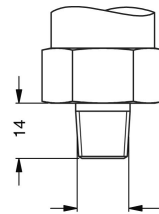
1/4" NPT
